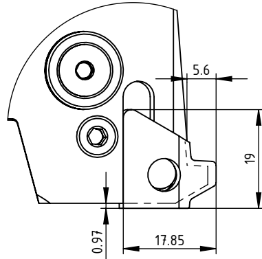
DETAIL C (1 : 1)
