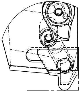
DETAIL C (1 : 1)
