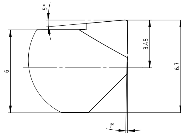
DETAIL A (6 : 1)
