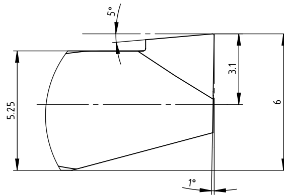
DETAIL A (6 : 1)
