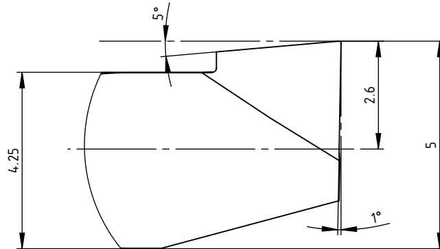
DETAIL A (8 : 1)
