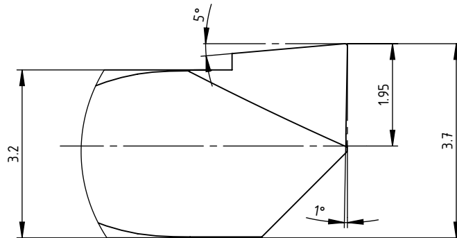
DETAIL A (10 : 1)
