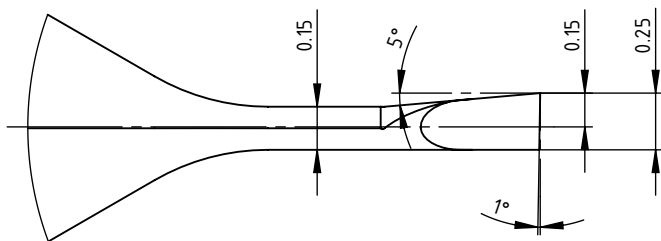
DETAIL A (30 : 1)
